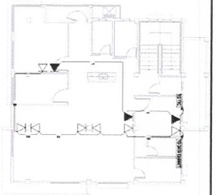
SECOND FLOOR TELEPHONE AND DATA LAYOUT SCALE 1:100
