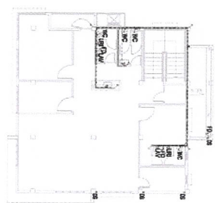
SECOND FLOOR PLUMBING LAYOUT
